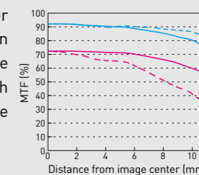
S: 20 lines/mm M: 20 lines/mm S: 40 lines/mm M: 40 lines/mm
