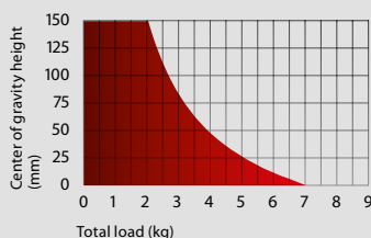
PAYLOAD DIAGRAM
