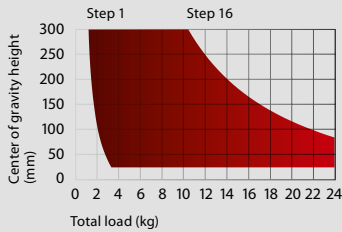
PAYLOAD DIAGRAM
